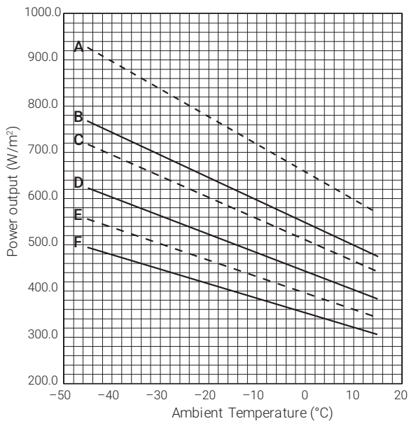
Raychem ArcticStep nominal power output at 230 Vac (W/m²)
