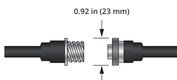
Cable construction
