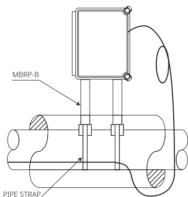
PIPE STRAP
