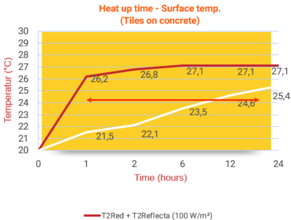
Figure 3: Heat up time scenarios
