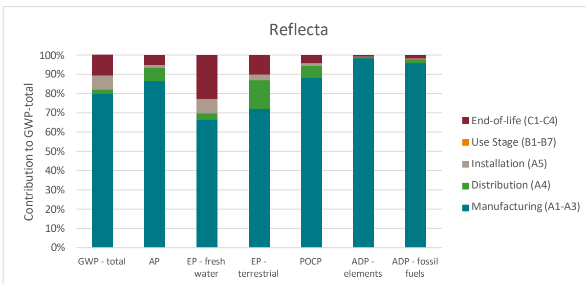
Figure 2: LCA Results for Reflecta, by life cycle stage
