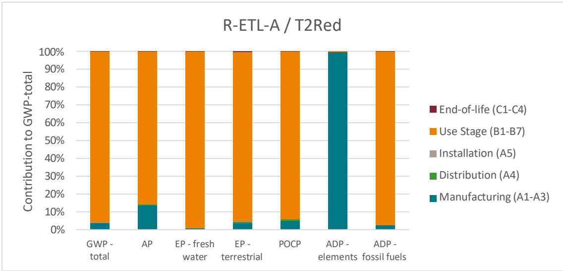
Figure 4: LCA Results for R-ETL-A / T2Red, by life cycle stage
