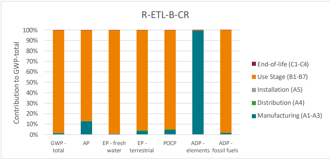
Figure 5: LCA Results for R-ETL-B (CR), by life cycle stage
