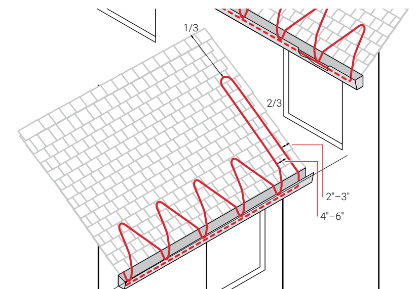
Fig. 13 Layout for a roof/wall intersection.
