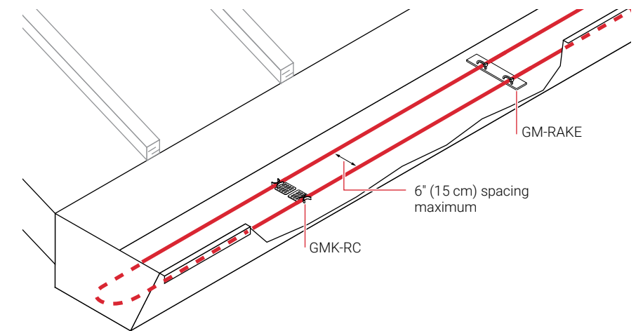
Fig. 23 GMK-RC clip in a gutter
