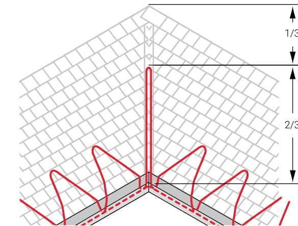
Fig. 12 Layout for a roof valley
