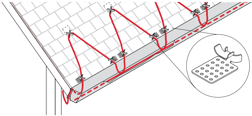
Fig. 18 GMK-RC clip attachment
