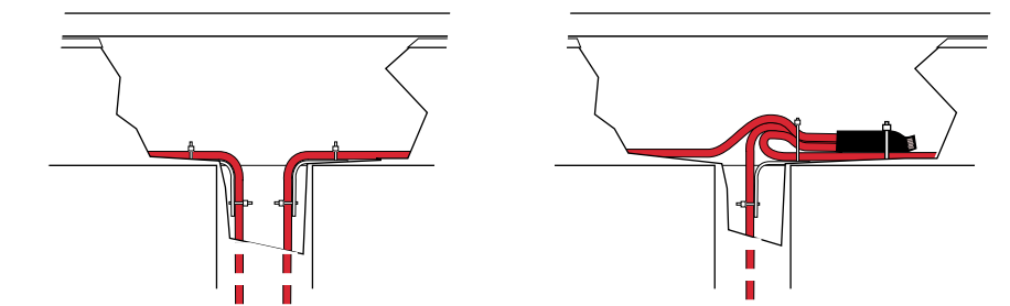
Fig. 24 GM-RAKE downspout hangers
