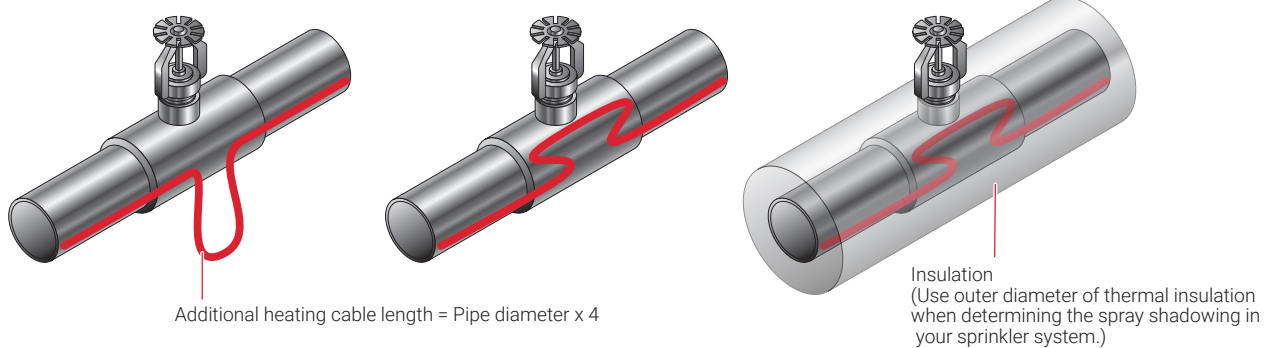
Sprinkler head with sprig
