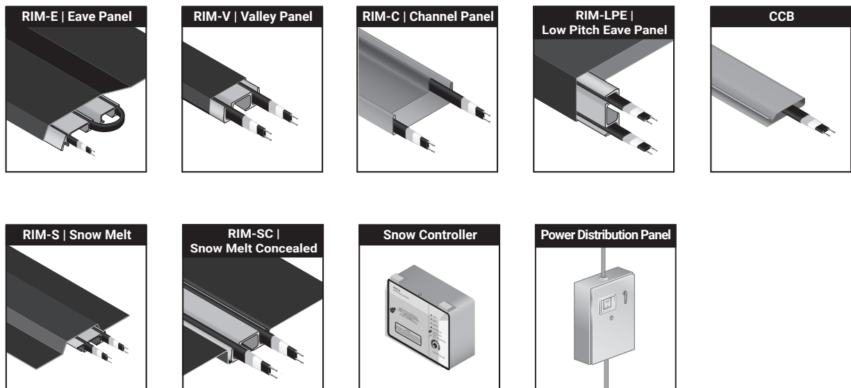
Fig. 1 Typical RIM System
