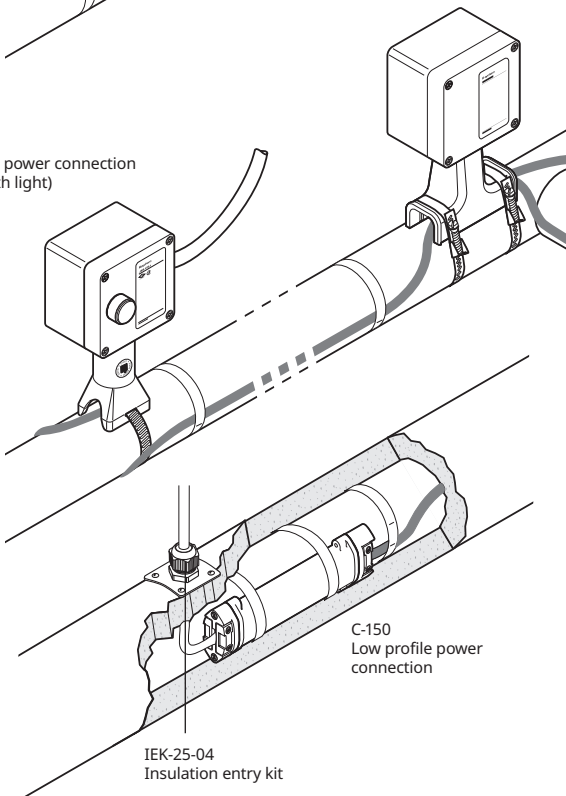
T-100 Tee or splice connection
