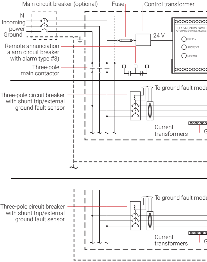
Figure 47: SMPG3 power distribution and control panel
