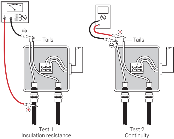
Figure 48: Insulation resistance and continuity test
