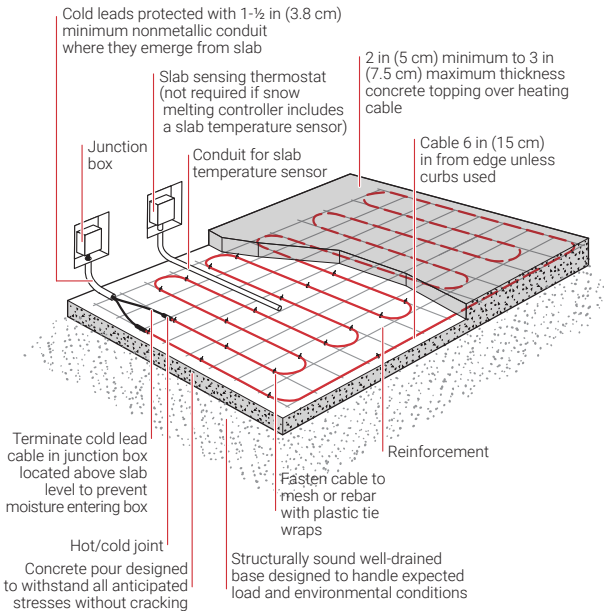
Figure 14: Single-pour concrete
