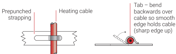
Figure 12: Method of bending tabs on prepunched strapping
