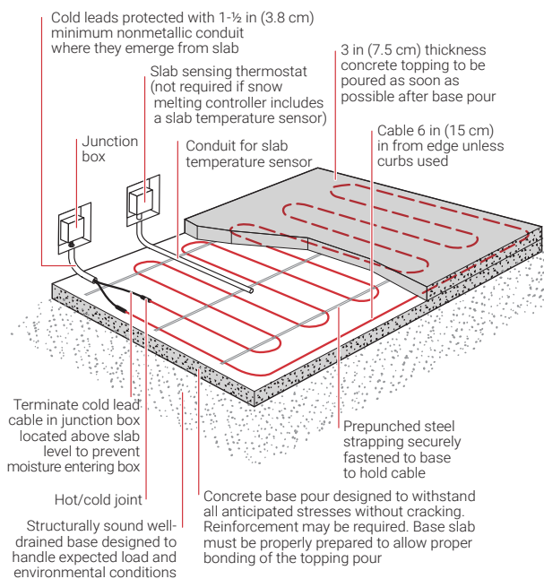
Figure 15: Two-pour concrete
