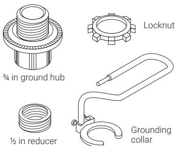
Figure 25: Typical ground hub
