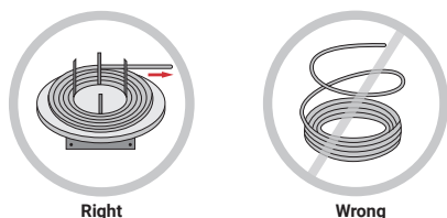
Figure 4: Unreeling/uncoiling cable
