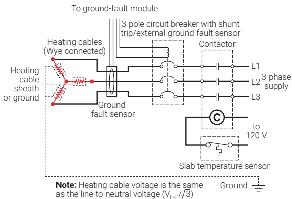
Figure 44: Thermostat control of balanced 3Ø Wye connected heating cables with contactor
