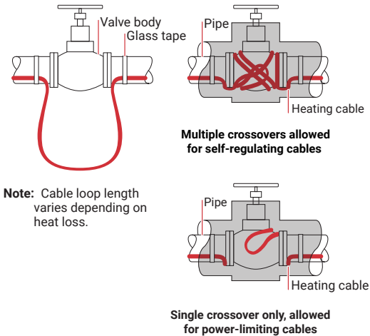
Figure 10: Valve
