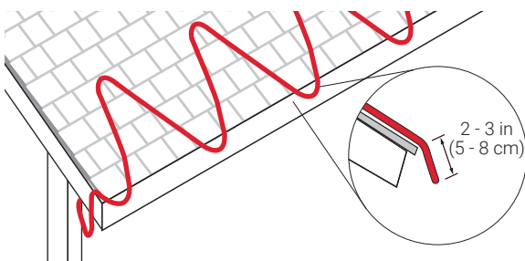
Figure 8: Layout for heated drip loops
