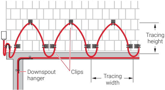
Figure 3: Front view of roof with IceStop system
