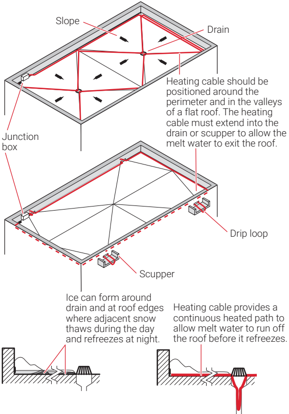
Figure 7: Layout on a flat roof
