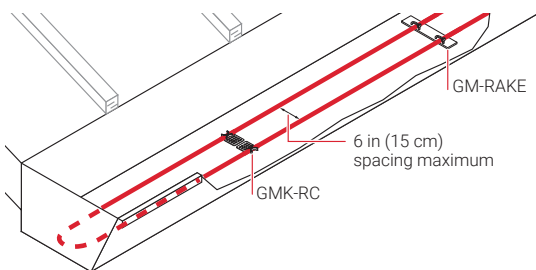
Figure 13: Layout in wide gutters—6 to 12 in wide
