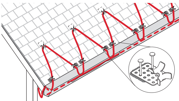
Figure 17: GMK-RC mechanical attachment
