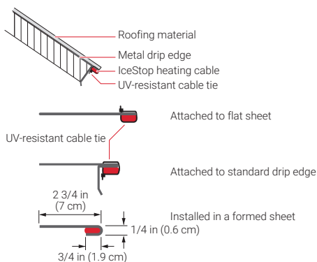
Figure 24: Heated drip edge attachment guidelines
