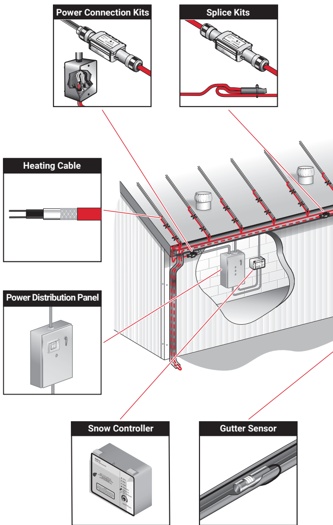
Figure 1: IceStop Roof and Gutter De-Icing System
