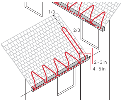
Figure 11: Layout for a roof/wall intersection
