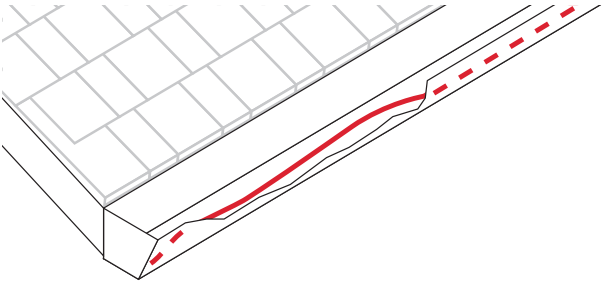
Figure 12: Layout in standard gutters—up to 6 in (16 cm) wide
