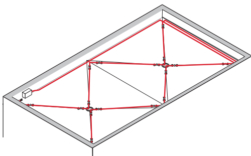
Figure 21: Belt loop approach on a flat roof
