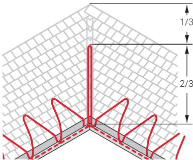
Figure 10: Layout for a roof valley
