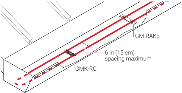
Figure 22: GMK-RC clip on a gutter
