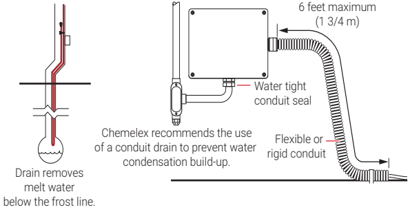
Figure 14: Installation of IceStop cable in trench drains
