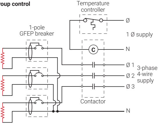
Figure 26: Typical controller wiring—multiple circuit
