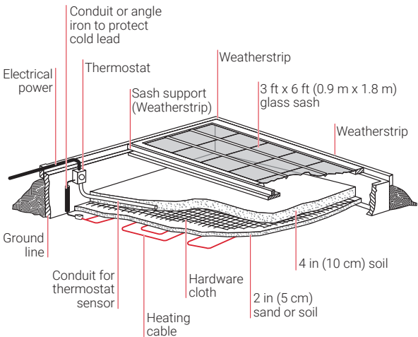
Figure 27: Typical soil heating installation
