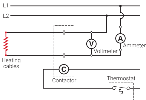
Figure 46: Using voltmeter and ammeter to measure voltage and current in a single-phase circuit
