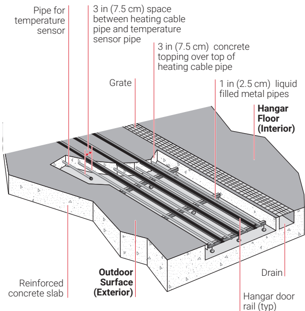
Figure 19: Typical hangar door deicing installation
