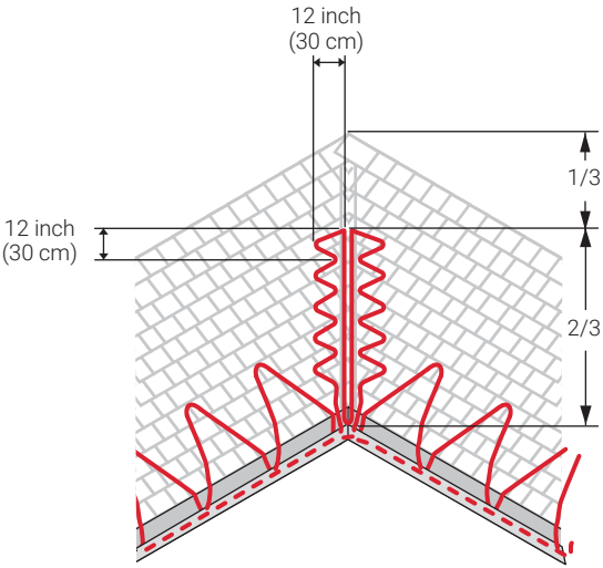
Figure 12: Alternate layout for valley
