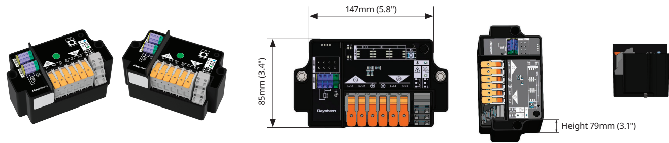
Figure 1: Dimensions of Elexant 3500i Module
