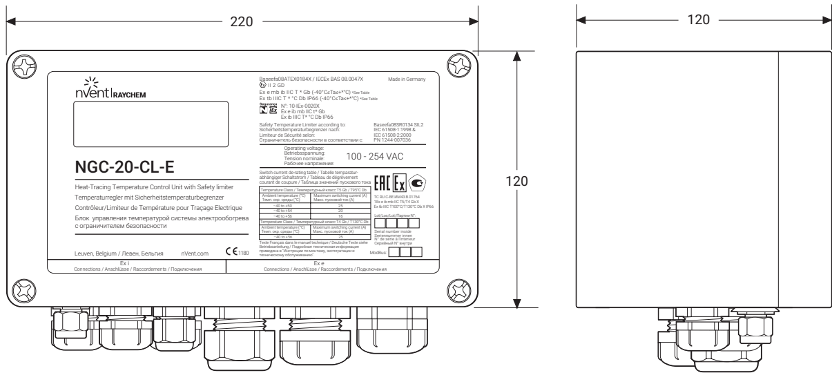
Figure 1: Dimensions NGC-20-C(L)-E
