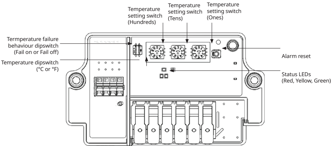
Figure 4: Elexant 3500i standard and alarm variant digital switches and rotary dials
