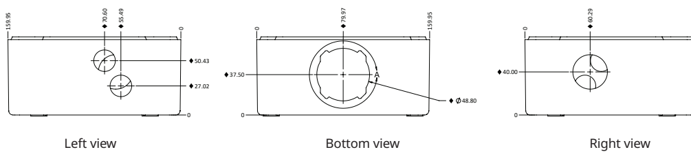
Figure 1: Elexant 3500i hub entry locations
