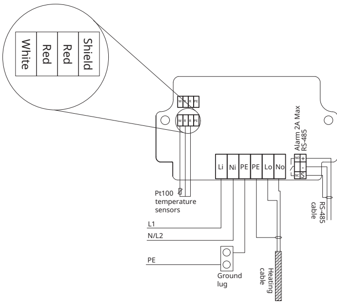
Figure 2: Wiring diagram
