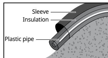
On rocky or inclined surfaces and where the pipe enters the lake, protect with oversized plastic pipe 4 in (10 cm) diameter or larger
