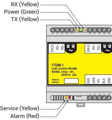
Figure 9. TTSIM-1 LED Locations
