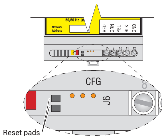
Figure 8. Reset Pads
