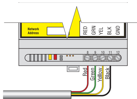
Figure 6. Sensing Cable Connections
