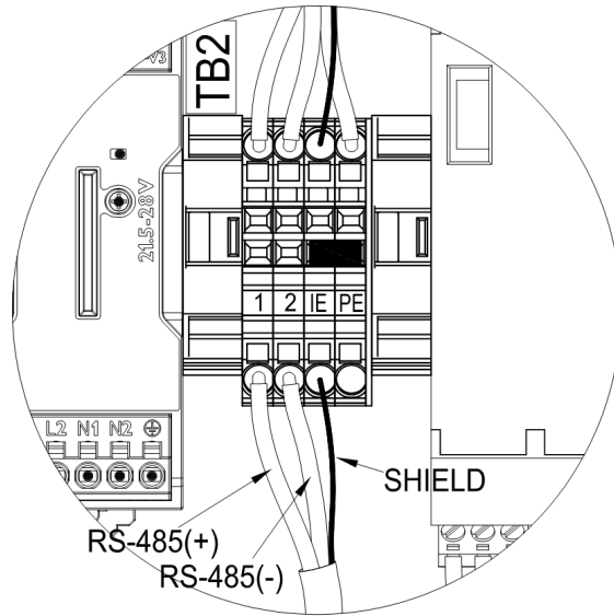
Figure 3 - RS-485 Connections
