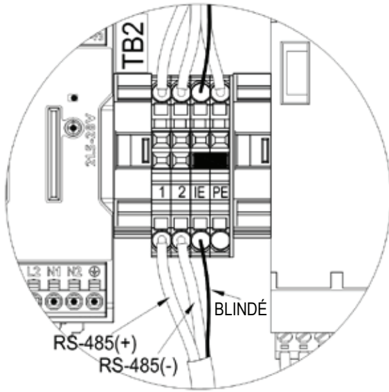
Figure 3 - Connexions RS-485
