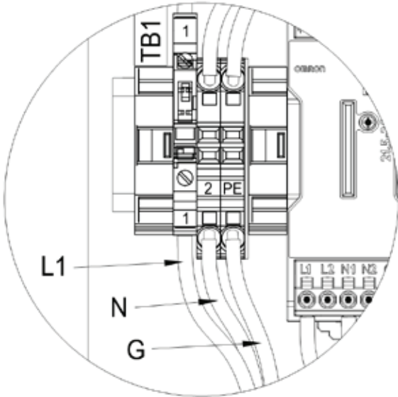
Figure 2 - Input Power
